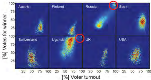
FIG. 1. Election fingerprints: 2-d histograms of the number of electoral districts for a given voter turnout (x-axis) and the percentage of votes (y-axis) for the winning party (or candidate) in recent elections from eight different countries (from left to right, top to bottom: Austria, Finland, Russia, Spain, Switzerland, Uganda, UK and USA) are shown. Color represents the number of electoral districts. Districts usually cluster around a given turnout and voting level. In Uganda and Russia these clusters are ‘smeared out’ to the upper right region of the plots, reaching a second peak at a 100% turnout and a 100% of votes (red circles). In Finland the main cluster is smeared out into two directions (indicative of voter mobilization due to controversies surrounding the True Finns). In the UK the fingerprint shows two clusters stemming from rural and urban areas (see SOM).
