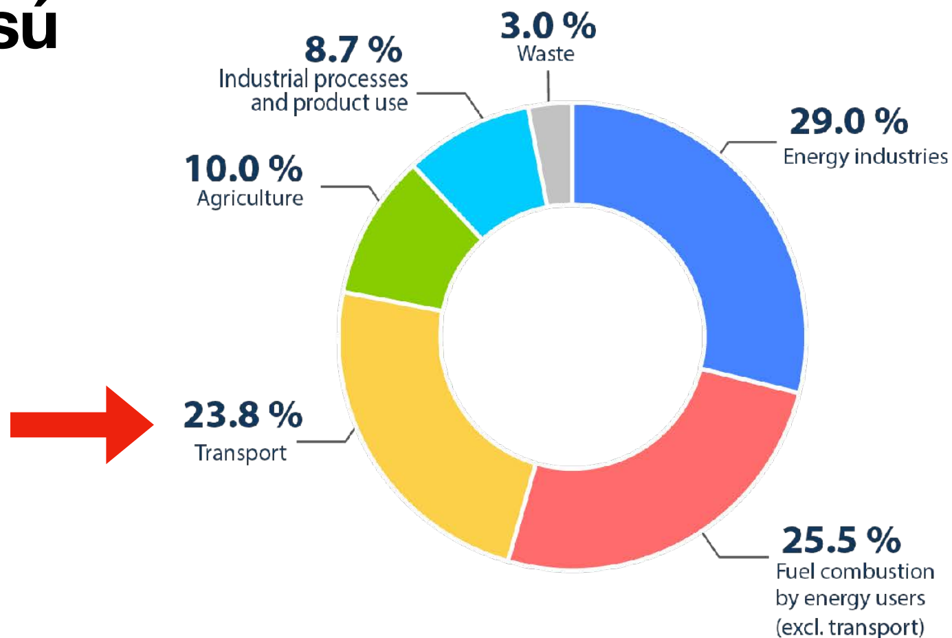
Share of EU greenhouse gas emission by source, 2017
