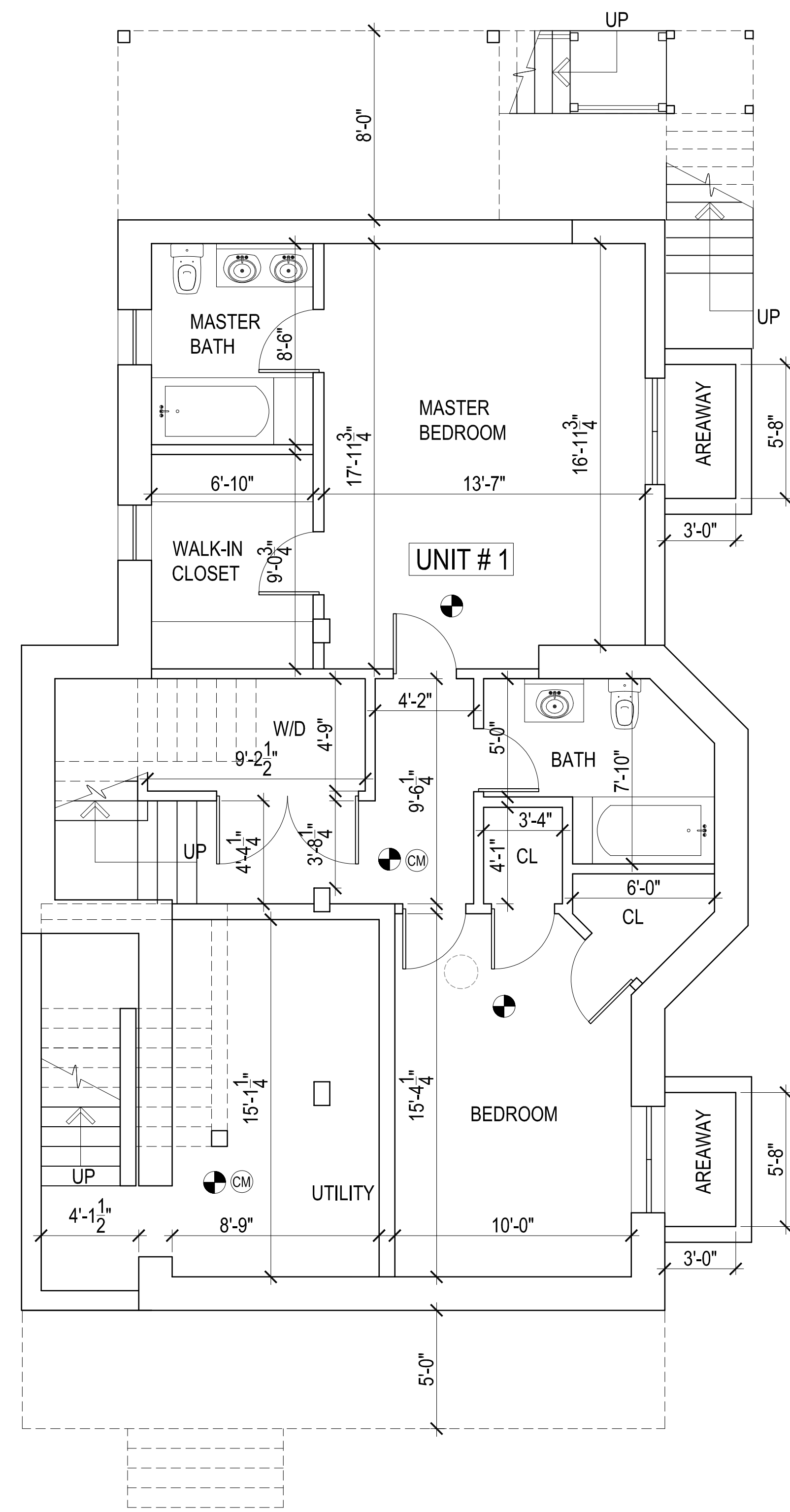
BASEMENT PLAN UNIT # 1 = 934 S.F.
