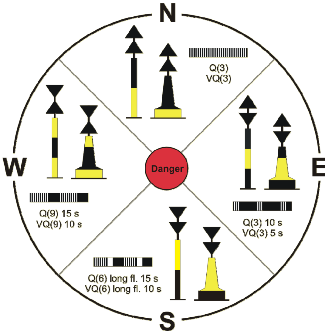
IALA Cardinal Buoyage System
